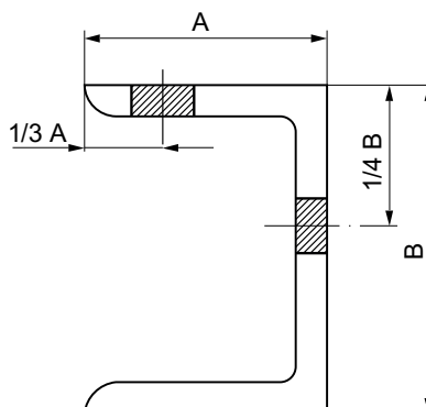
Figure 5 : Sections
