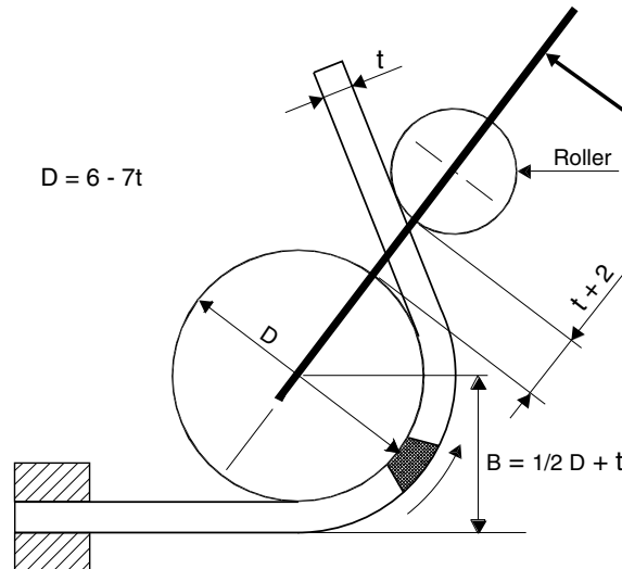
Figure 2 : Wrap around bend test
