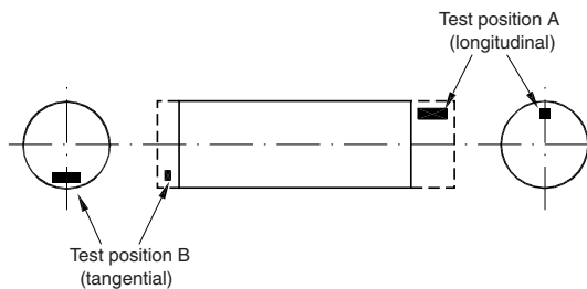
Figure 2 : Flanged shaft
