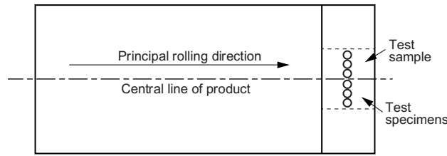
Figure 1 : Plate and wide flat sampling position
