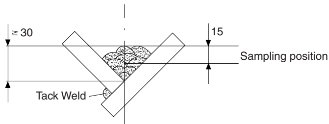
Figure 1 : Deposited weld metal test assembly
