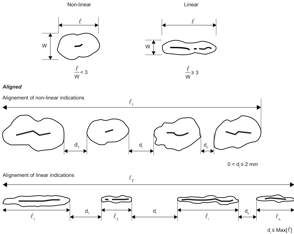
Figure 7 : Shape of indications
