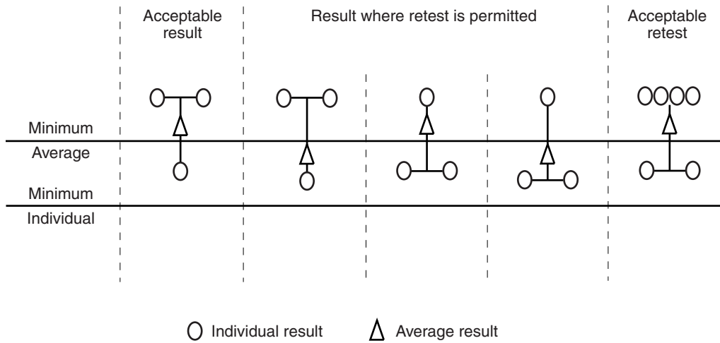
Figure 4 : Diagram showing acceptance / rejection and retest criteria
