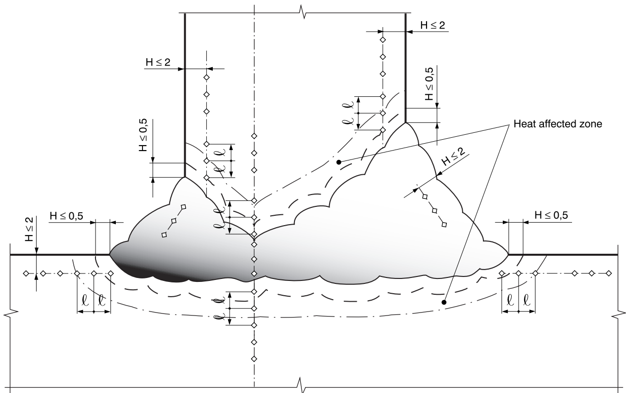
Figure 8 : Hardness indentations
