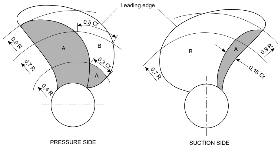
Figure 6 : Severity zones in blades with skew angles > 25°
