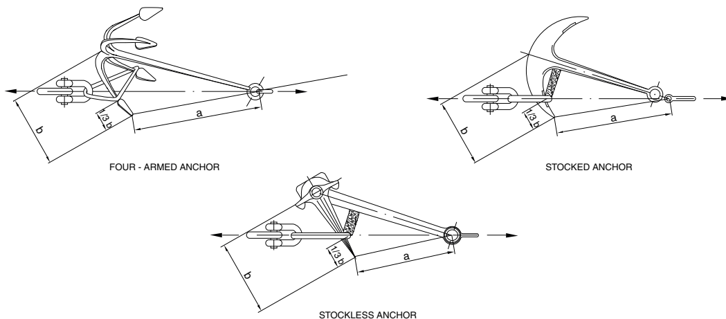
Figure 2 : Proof load test
