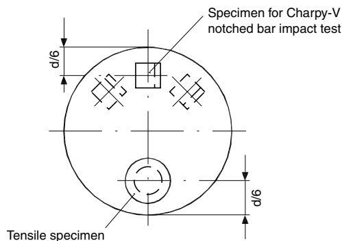
Figure 1 : Sampling of chain cable steel
