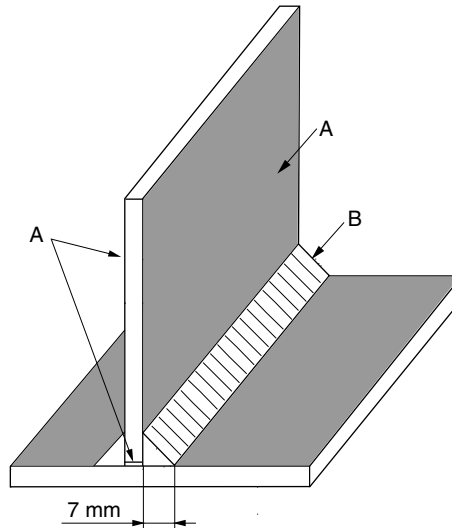
Figure 1 : Typical T welded sample
