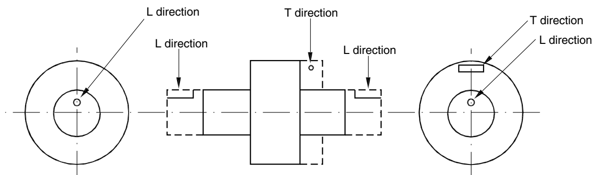
Figure 1 : Turbine rotor
