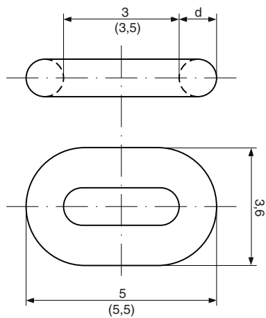
Figure 1 : Studless link for studless chain cable
