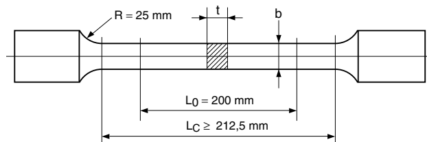
Figure 2 : Non proportional flat specimen
