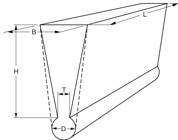
Figure 1 : Keel block test sample casting
