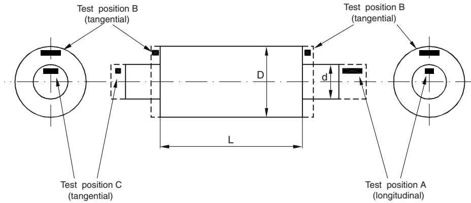
Figure 1 : Pinions
