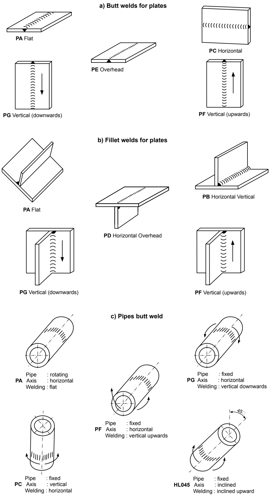
Figure 13 : Welding positions according to ISO Standard
