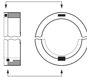
Figure 4 : Forged rings
