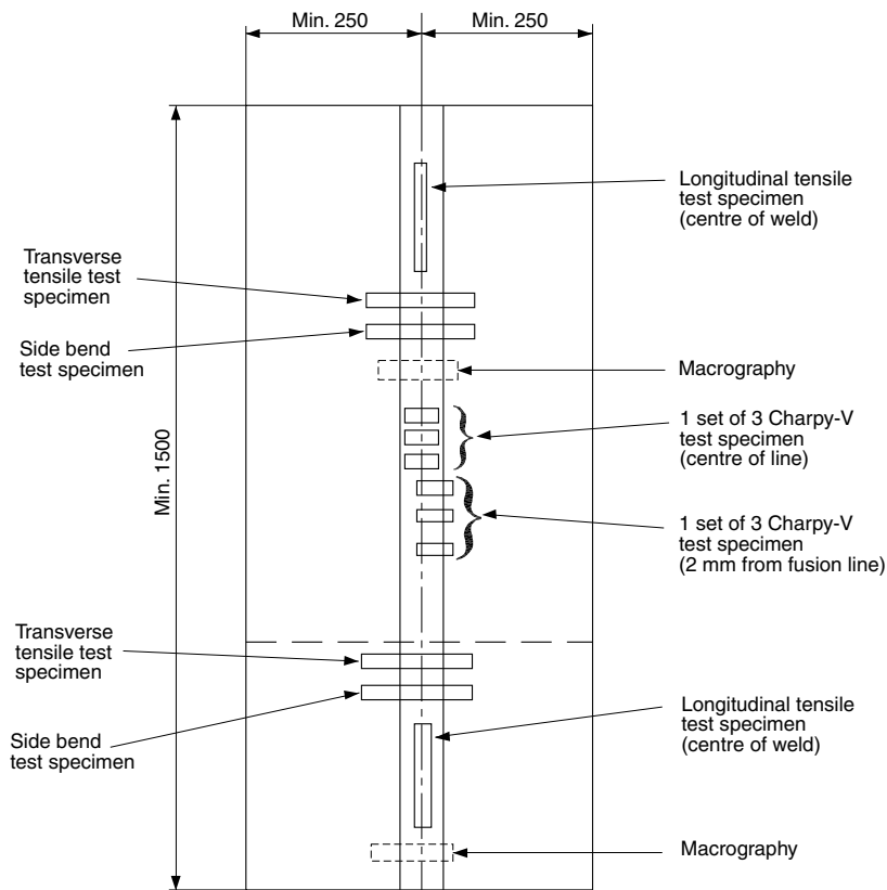
Figure 1 : Butt weld test assembly for electrogas and electroslag welding
