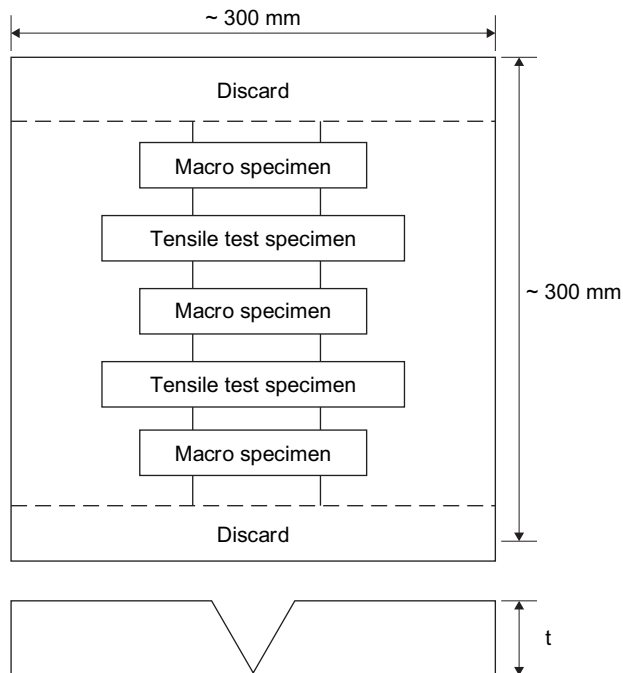
Figure 3 : Test specimen
