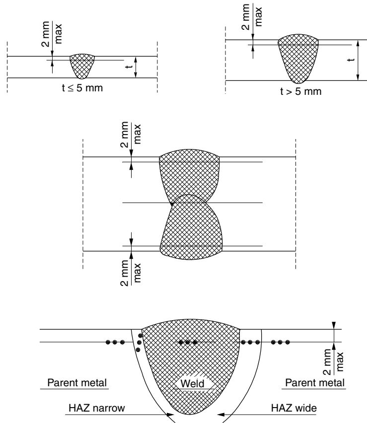
Figure 7 : Examples of hardness indentations
