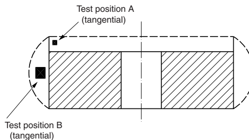
Figure 2 : Gear wheel
