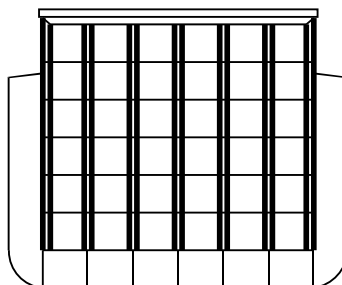
Figure 1 : Containers in holds within cell guides
