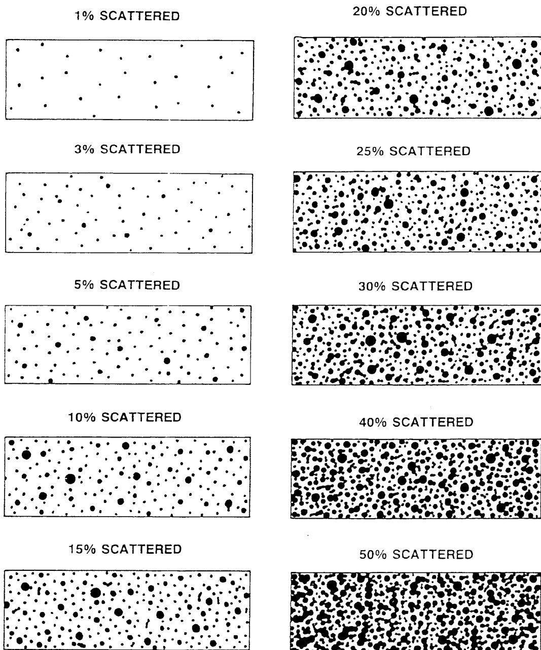
Figure 4 : Pitting intensity diagrams (from 1% to 50% intensity)
