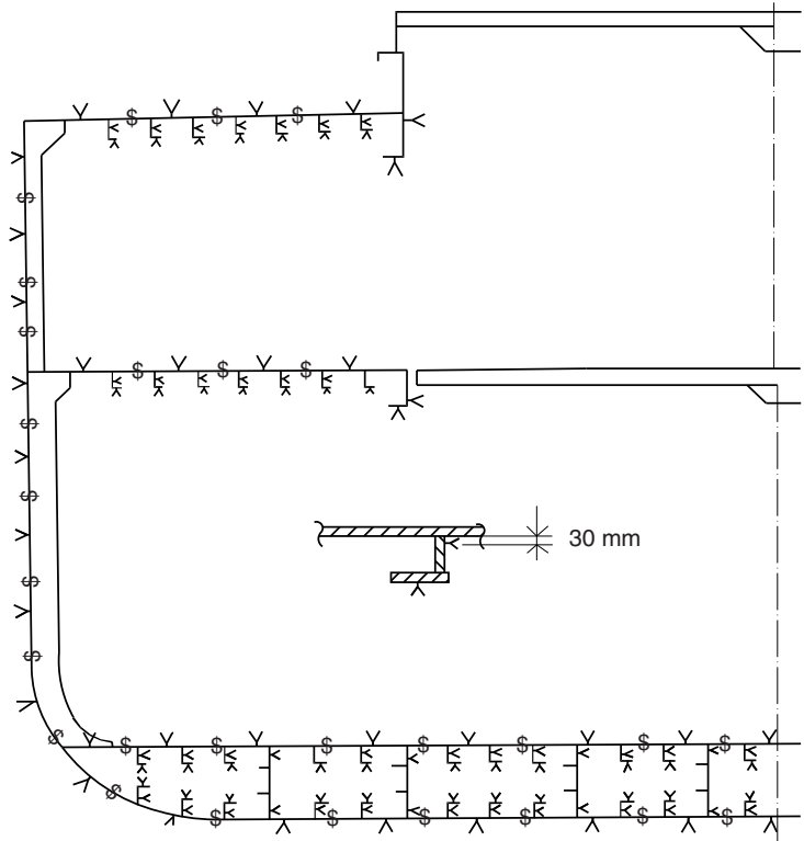
Figure 1 : Transverse section of a military ship
