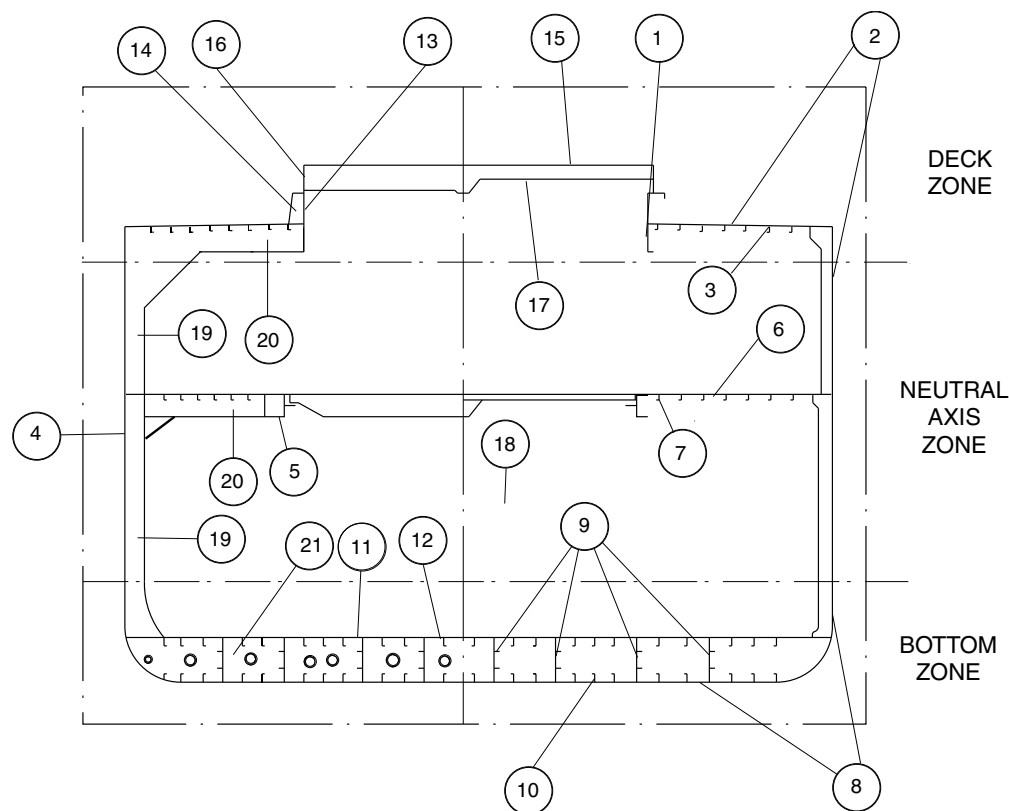
Figure 5 : Military ship: layout of items to be assessed
