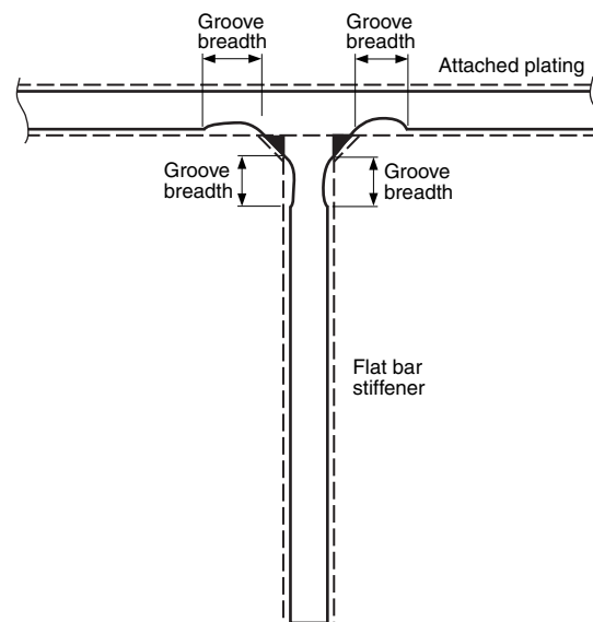
Figure 24 : Grooving corrosion
