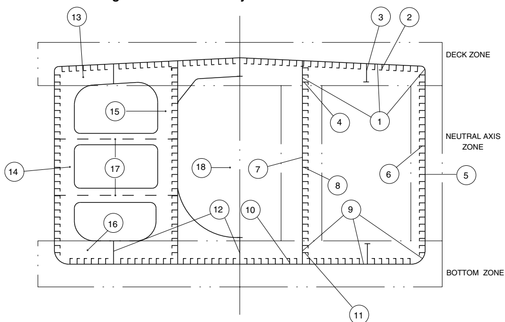
Figure 21 : Oil tanker: layout of items to be assessed
