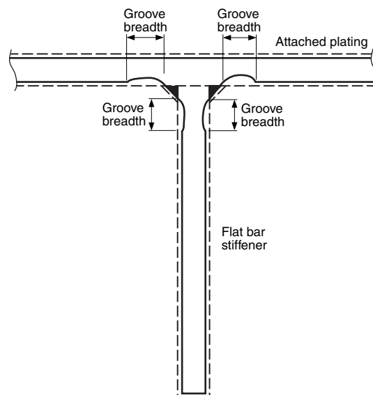
Figure 24 : Grooving corrosion
