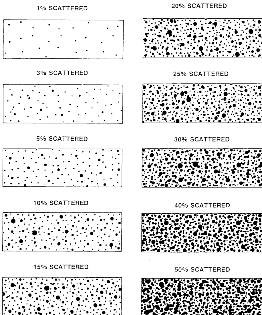
Figure 22 : Pitting intensity diagrams (from 1% to 50% intensity)
