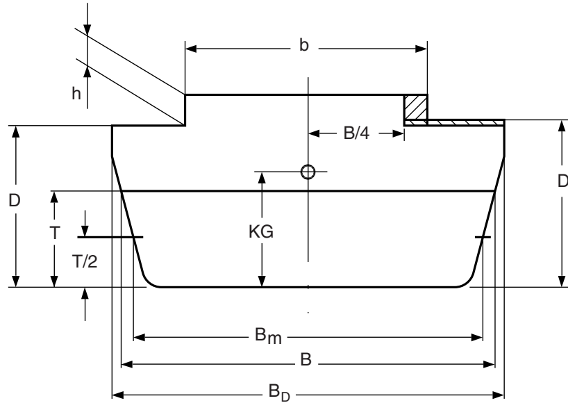
Figure 2 : Definition of dimensions
