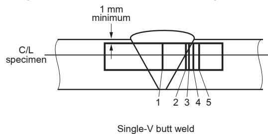
Figure 2 : Orientation of weld test specimen
