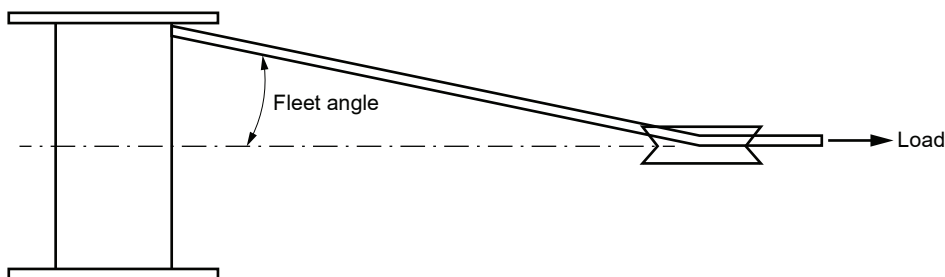
Figure 1 : Fleet angle
