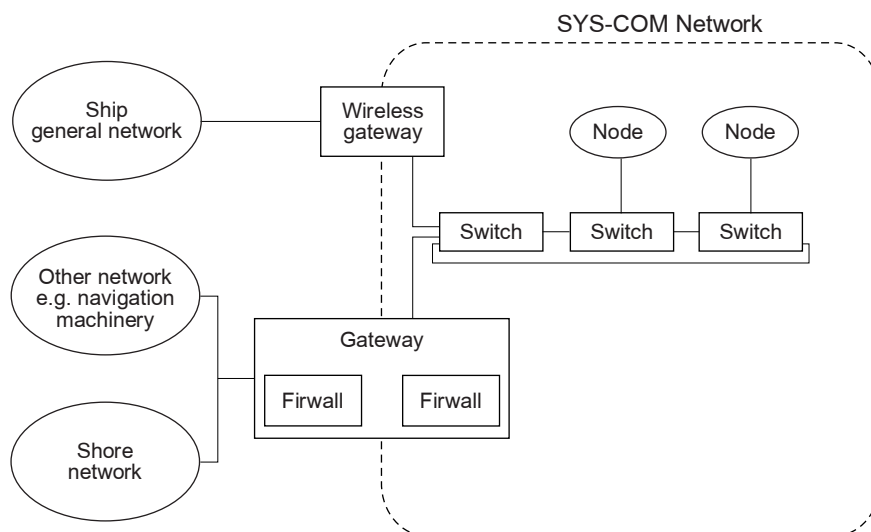
Figure 1 : Typical network architecture
