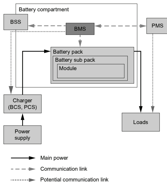
Figure 1 : Battery system considered
