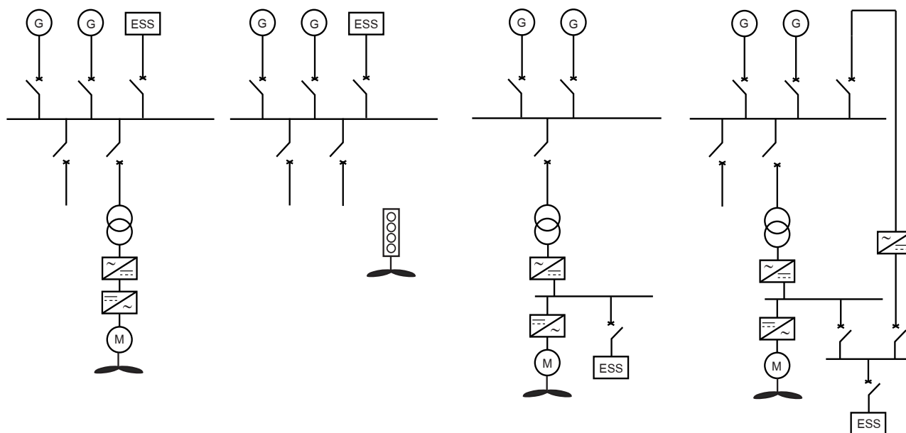
Figure 1 : Typical ESS supply arrangements
