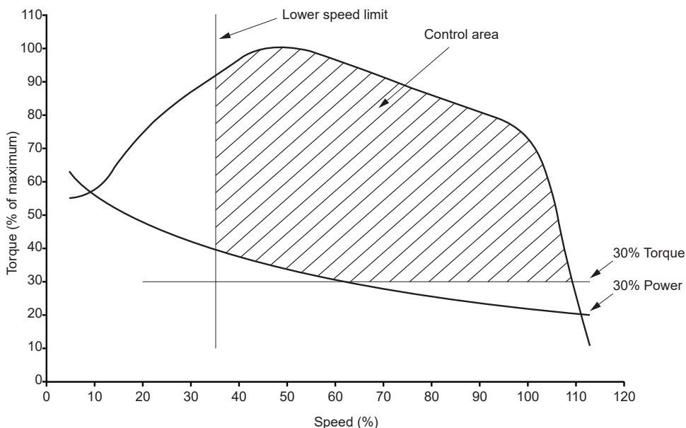
Figure 2 : Control area for variable speed propulsion engine
