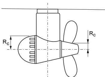
Figure 10 : Dimensions used for Rc
