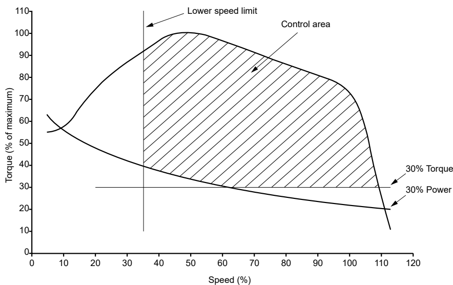
Figure 1 : Control area for variable speed auxiliary engines
