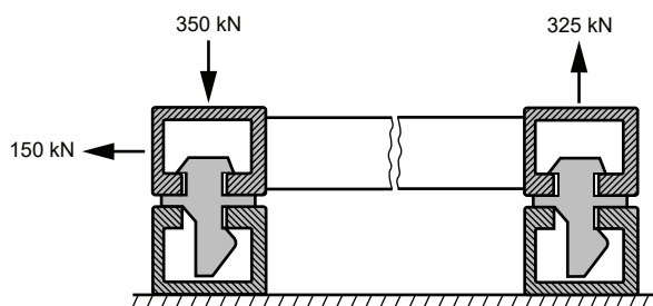
Figure 6 : Pull test
