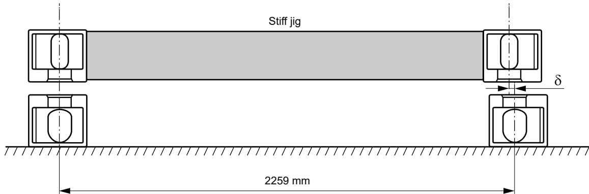
Figure 5 : Test rig
