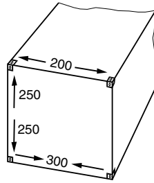
Figure 14 : Permissible transverse and vertical compressions on end and intermediate frames of 45' ISO containers
