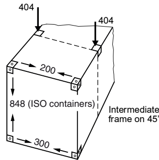
Figure 15 : Permissible vertical compression on frames of 45' ISO containers topped on 40' containers
