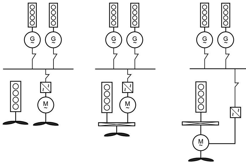
Figure 1 : Propulsion arrangements
