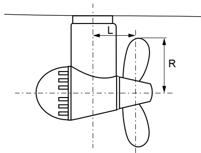
Figure 12 : Distance from the propeller plane to steering axis
