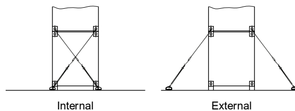
Figure 4 : Internal and external lashing
